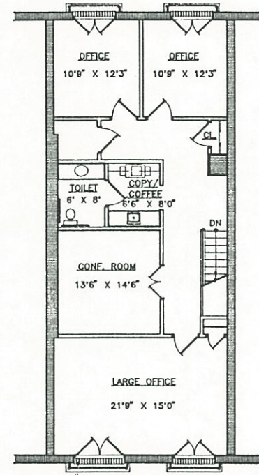
P L A N SECOND FLOOR
