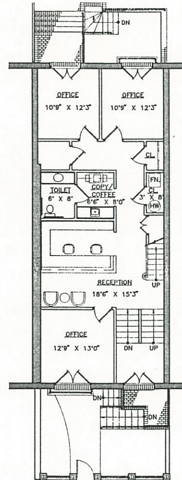
P L A N FIRST FLOOR
